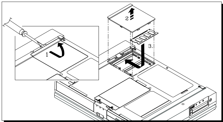
Figure 6-1: Removing the Memory Door and Installing the Memory Card
