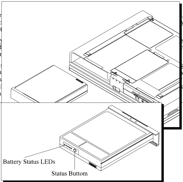
Figure 5-3: The Main Battery Module
