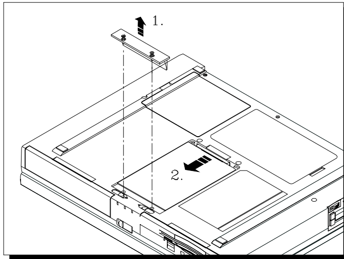
Figure 6-4: Removing the HDD Module (A)
