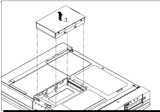
Figure 6-5: Removing the HDD Module (B)
