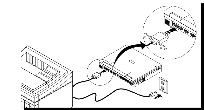
Figure 4-2: Connecting a Printer to the Notebook's Parallel Port
