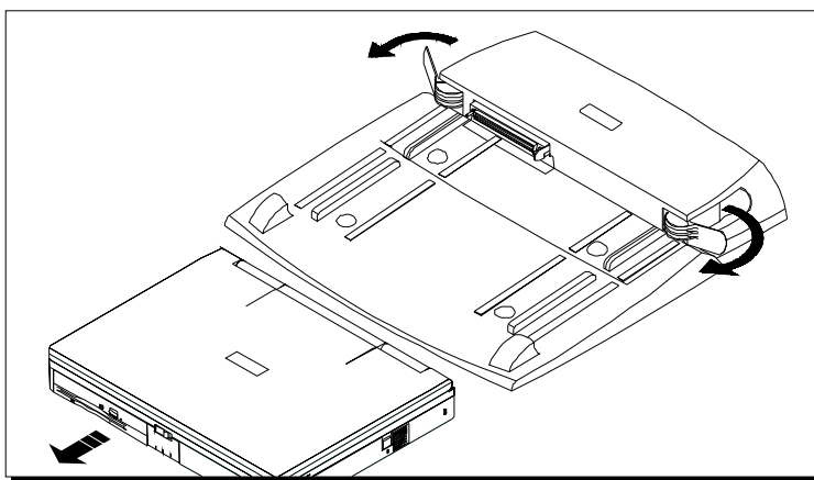
Figure 6-10: Removing the Notebook from the I/O Replicator
