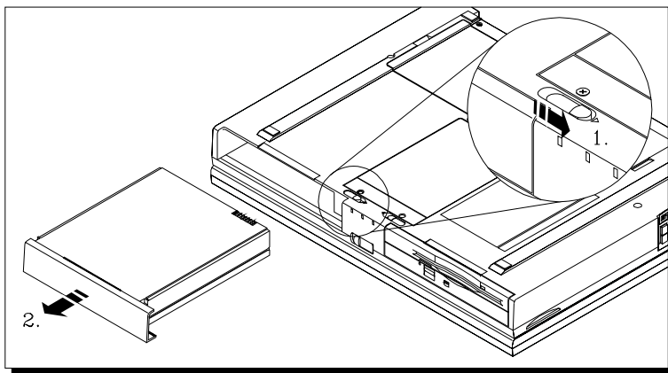
Figure 5-4: Removing the Battery Pack
